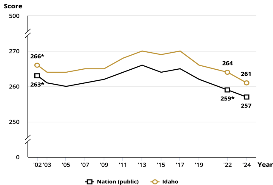
Graph 1.3 NAEP – Grade 8
